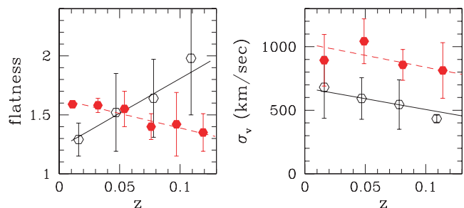
Figure 6. The redshift–flatness (left-hand panel) and redshift–velocity dispersion (right-hand panel) mean correlations for the poorest (open symbols and continuous lines) and the richest (solid symbols and dashed lines) cluster subsamples.
