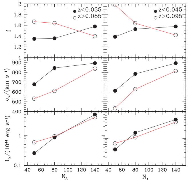
Figure 9. The variation with richness of the mean cluster dynamics proxies for two sets of well-separated redshift bins (indicated in the plot).
