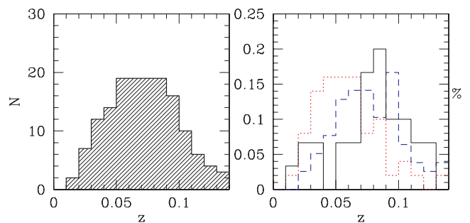
Figure 1. Left-hand panel: the redshift distribution of our cluster sample. Right-hand panel: the normalized redshift distribution of three subsamples based on different cluster richness. Clusters with 20 < N_A < 50 , 50 \leq N_A < 80 and N_A \geq 80 are represented by the dotted, dashed and continuous line histograms, respectively.
