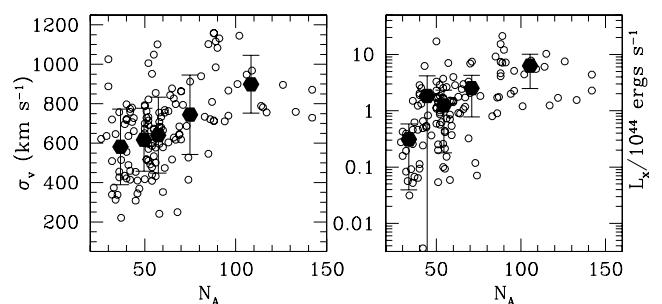
Figure 2. The correlation between Abell galaxy count, N_A , and the cluster velocity dispersion (left-hand panel) and X-ray luminosity (right-hand panel) for our sample. The filled symbols correspond to the mean values in bins of N_A and uncertainties are 1\sigma .
