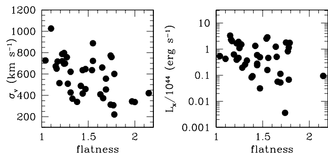
Figure 10. Correlation of two proxies for cluster dynamical state for the poorest subsample ( 20 < N_A < 50 , z < 0.1 ). Left: the dependence of cluster velocity dispersion on cluster flatness. Right: the dependence of cluster X-ray luminosity on cluster flatness.
