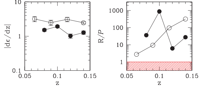
Figure 8. Left-hand panel: the dependence of the cluster ellipticity evolution rate on the limiting sample redshift. Filled and open points correspond to the richest and poorest samples, respectively. Note that since d\epsilon/dz is negative for the richest subsample, we plot its absolute value. Right-hand panel: a measure of the corresponding significance of the estimated d\epsilon/dz (see main text). Values corresponding to R/P \lesssim 1 (shaded region) are not significant.
